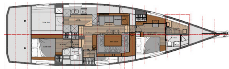
STANDARD VERSION – 2 CABINS
